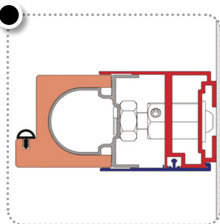
WALL-MOUNTED HORIZONTAL SECTION
