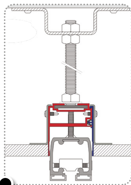
FALSE CEILING-MOUNTED VERTICAL SECTION
