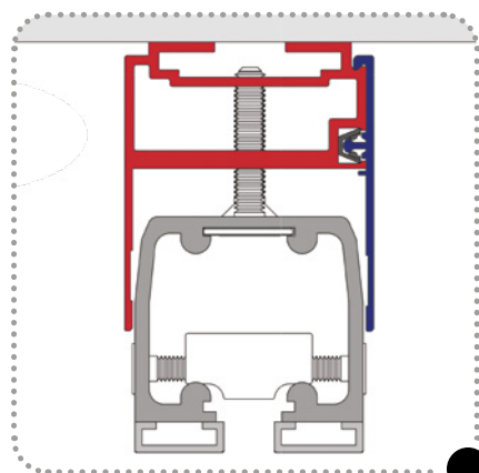
CEILING-MOUNTED VERTICAL SECTION
